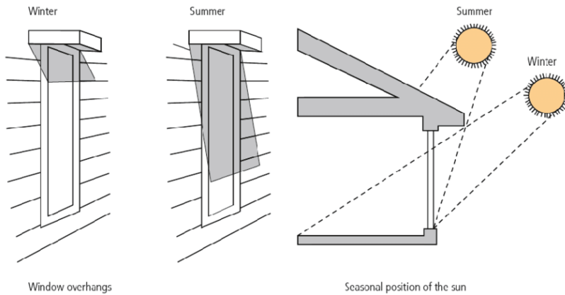
Figure 2. Principal of fixed shading and differences between winter and summer (Source: Akande et al., 2015)
